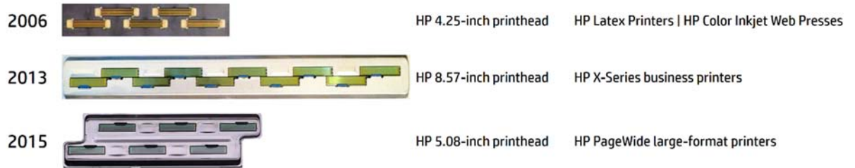
Figure 2. Three generations of printheads used in HP PageWide Technology
