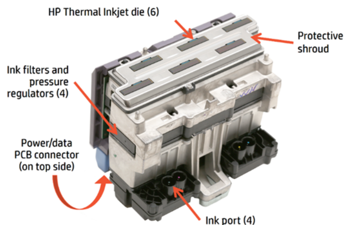
Figure 1. Printhead module used in HP PageWide large-format printers
